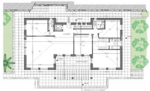
VILLA A - PIANO TERRA
